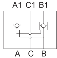
Circuit drawing 迴路圖
