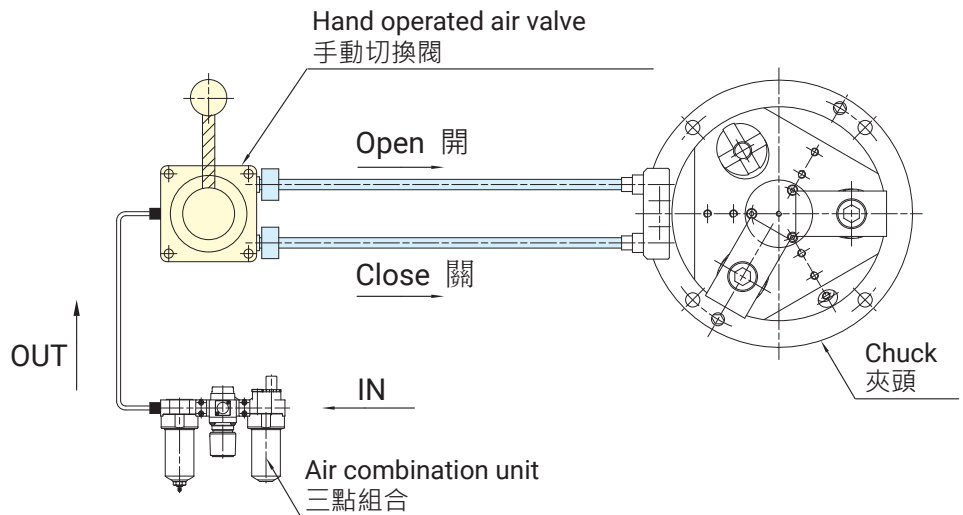
Assembly drawing 裝配圖
